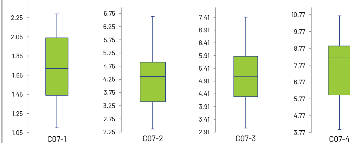
Box and Whisker Plots
